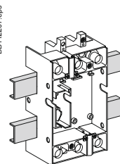
Mounting on rails.
