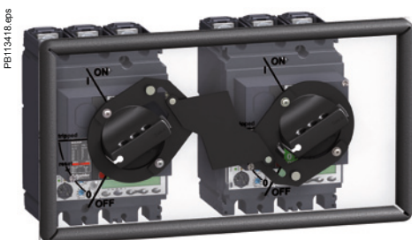
Interlocking of two devices with rotary handles.
