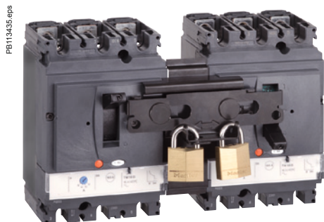
Interlocking of two or three toggle-controlled devices.
